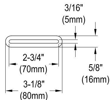
View B (Scale 5:1)
